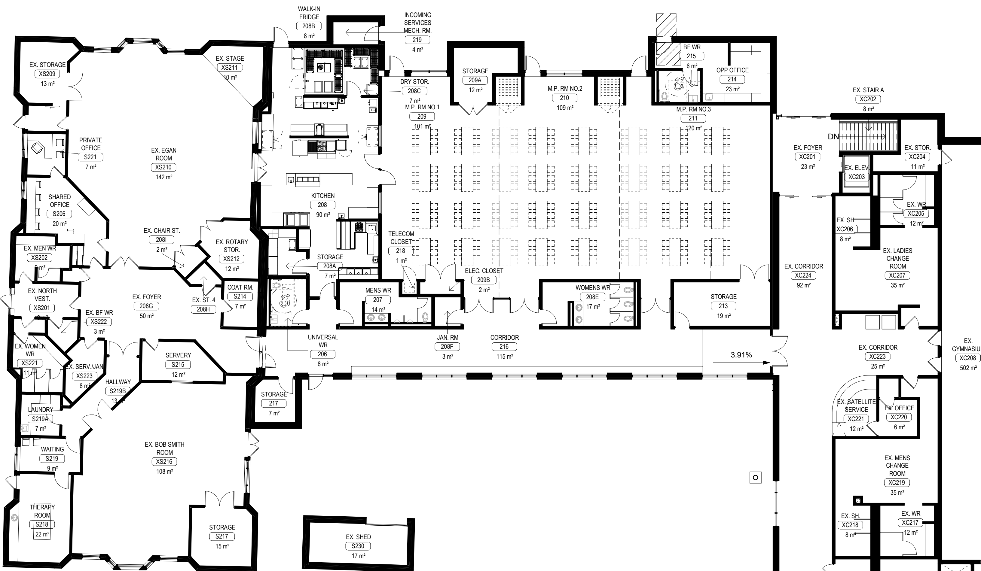
PRELIMINARY GROUND FLOOR PLAN
